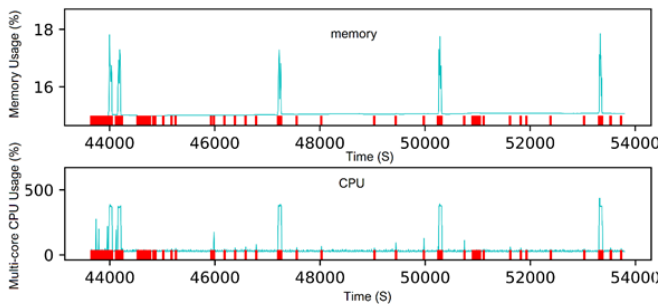
Figure 7. CPU and memory usage during the test period and five bug events in the Train Ticket case study. Detected anomalies depicted by red bars.
